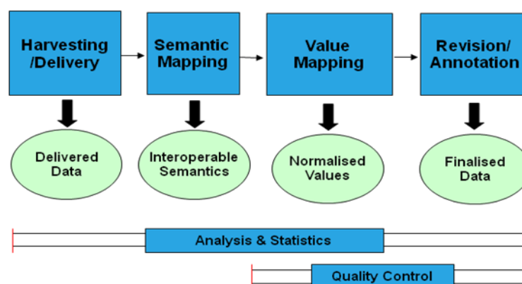
Figure 1. Ingestion workflow
